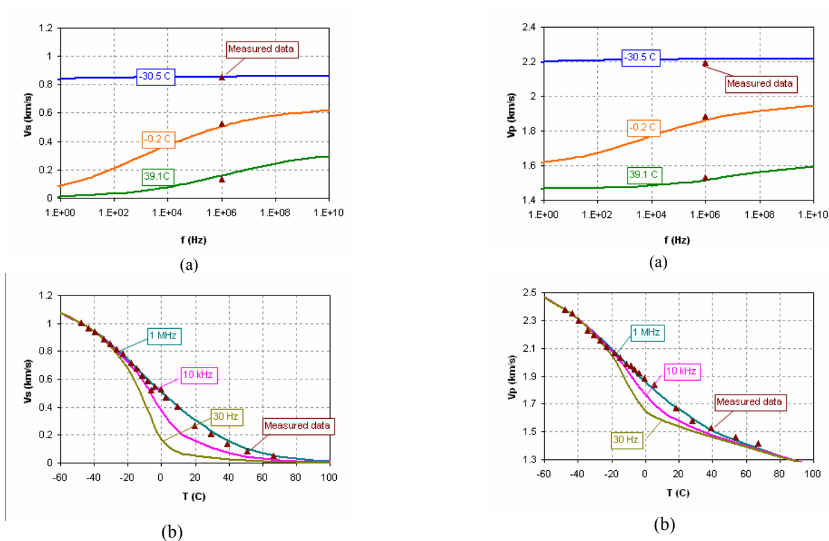
Fig. 5. Estimated P velocity vs. frequency for a heavy oil with API = 9.38.
