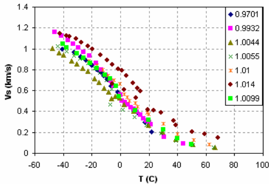
Fig. 2. Measured Vs as function of temperature.
