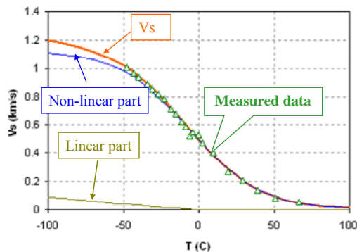
Fig. 3. Vs model vs. temperature (API = 9.38)
