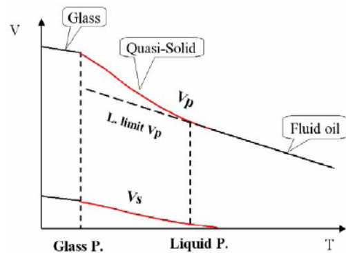
Fig. 1 Velocities of heavy oil in phase transition
